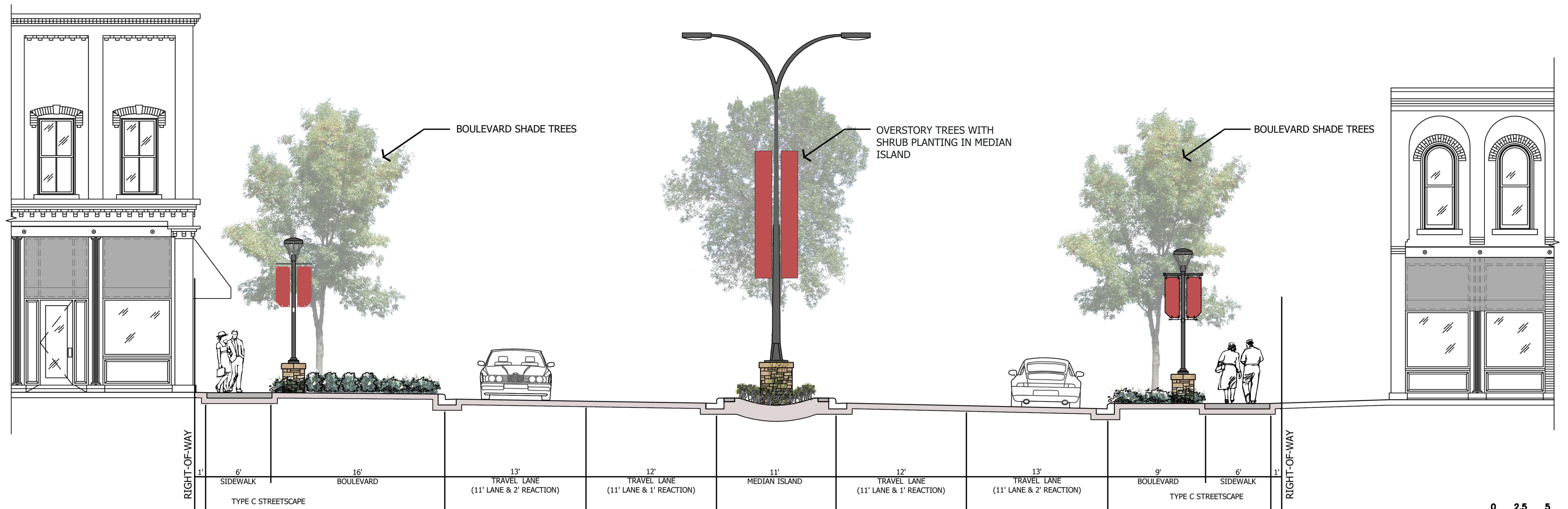
SECTION 'B - B' TYPICAL CROSS SECTION WITH OUT PARKING
