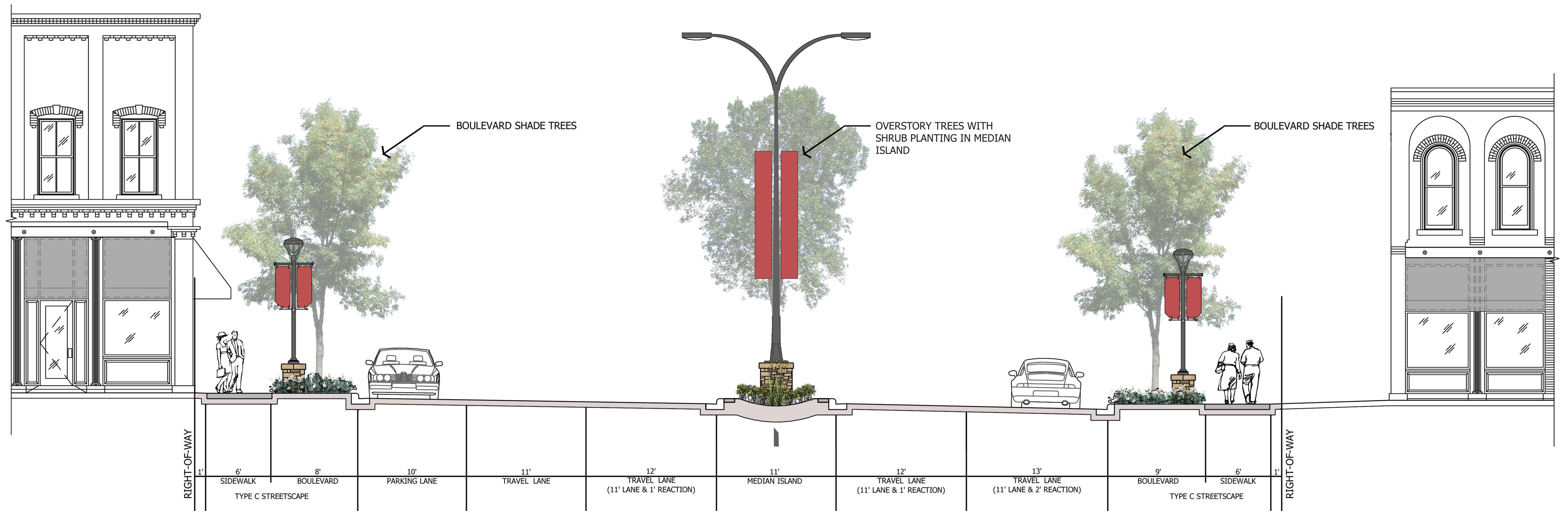
SECTION 'A - A' TYPICAL CROSS SECTION WITH PARKING
