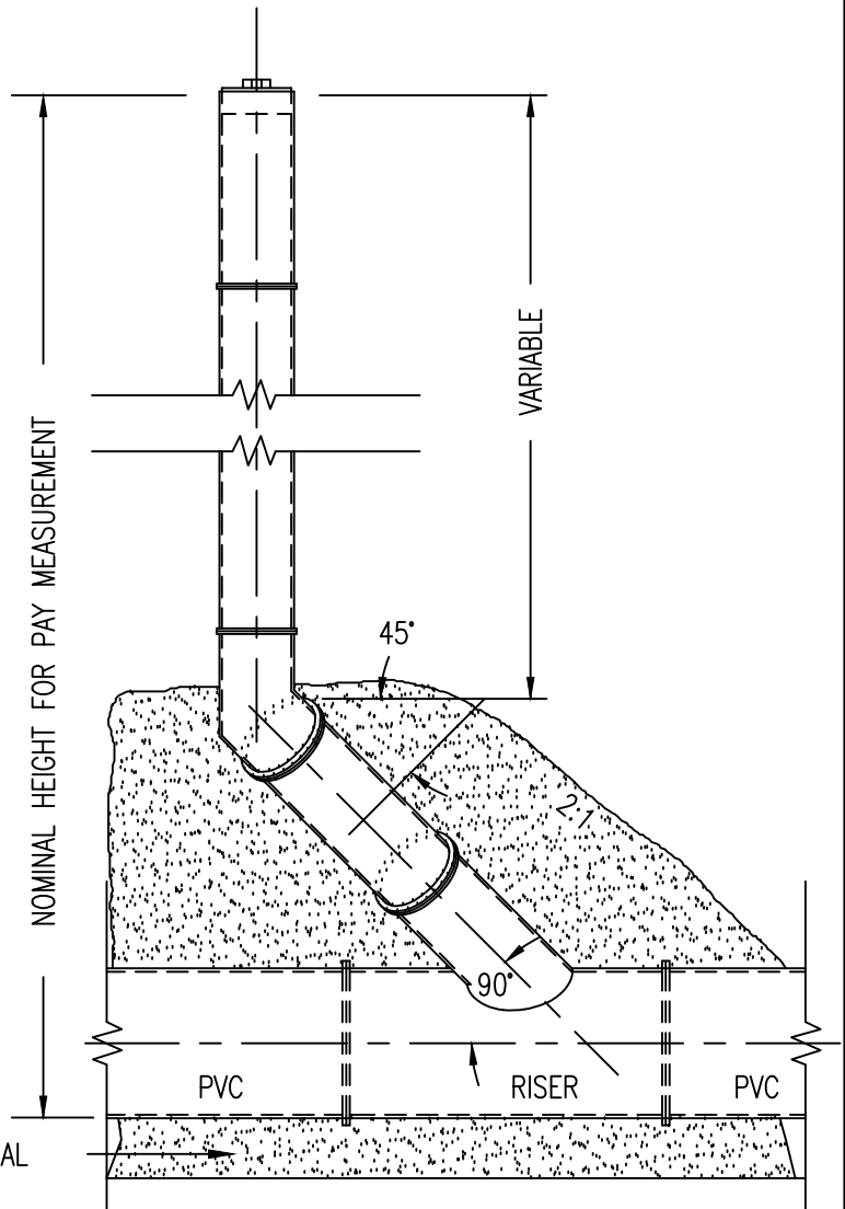
SIDE ELEVATION
