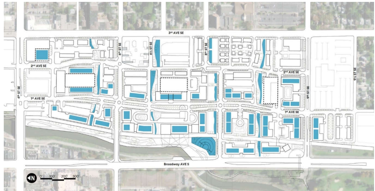
Figure 55: DWSE Small Area Plan – Stormwater System
